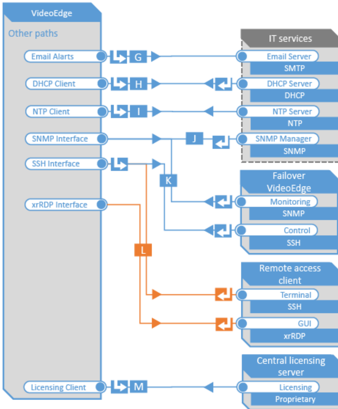
VideoEdge Data Flow Diagram (2 of 2)
