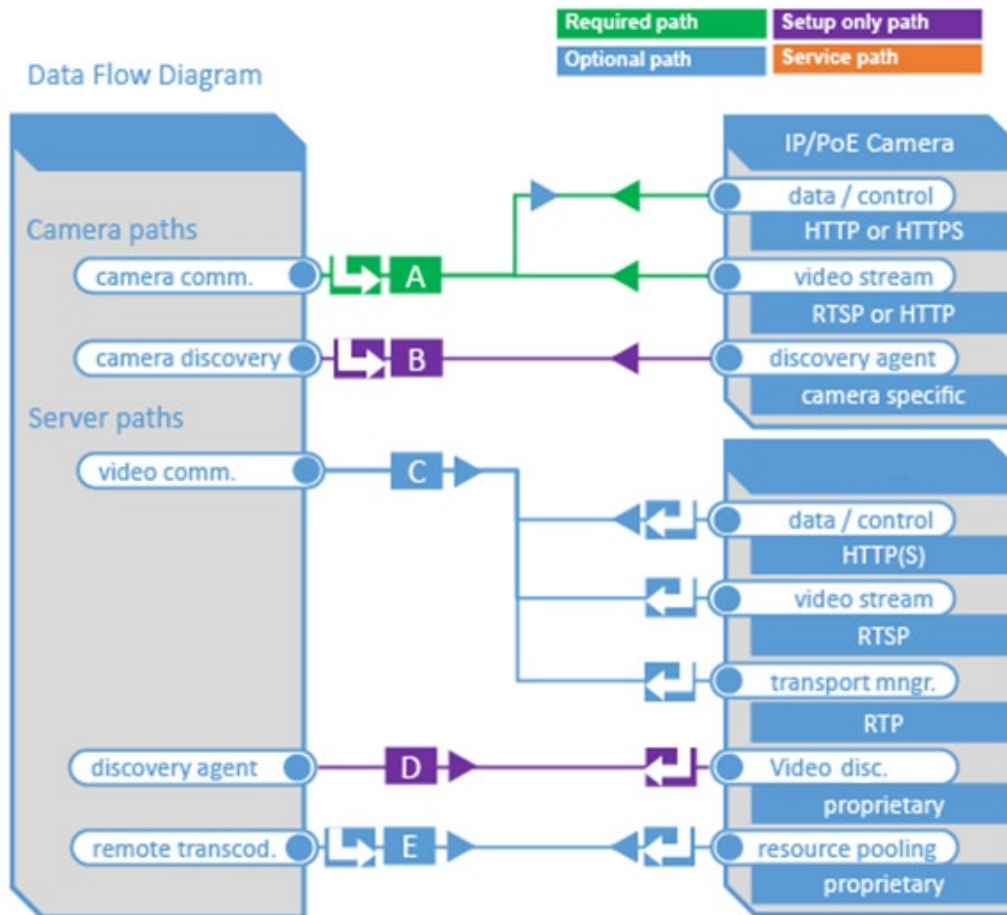
Figure 1.5.0 Sample Data Flow Diagram
